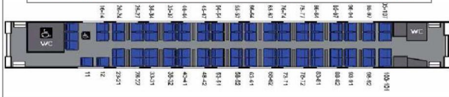
UICZ1 HK Carriage sketch (2nd class, central aisle, 70 seats, 3 seats and toilet for disabled passengers)
